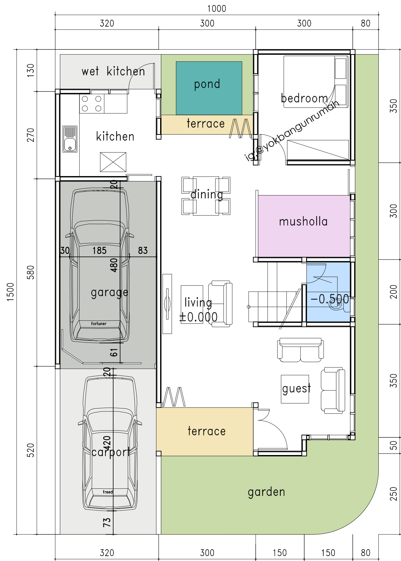
1st FLOORPLAN
