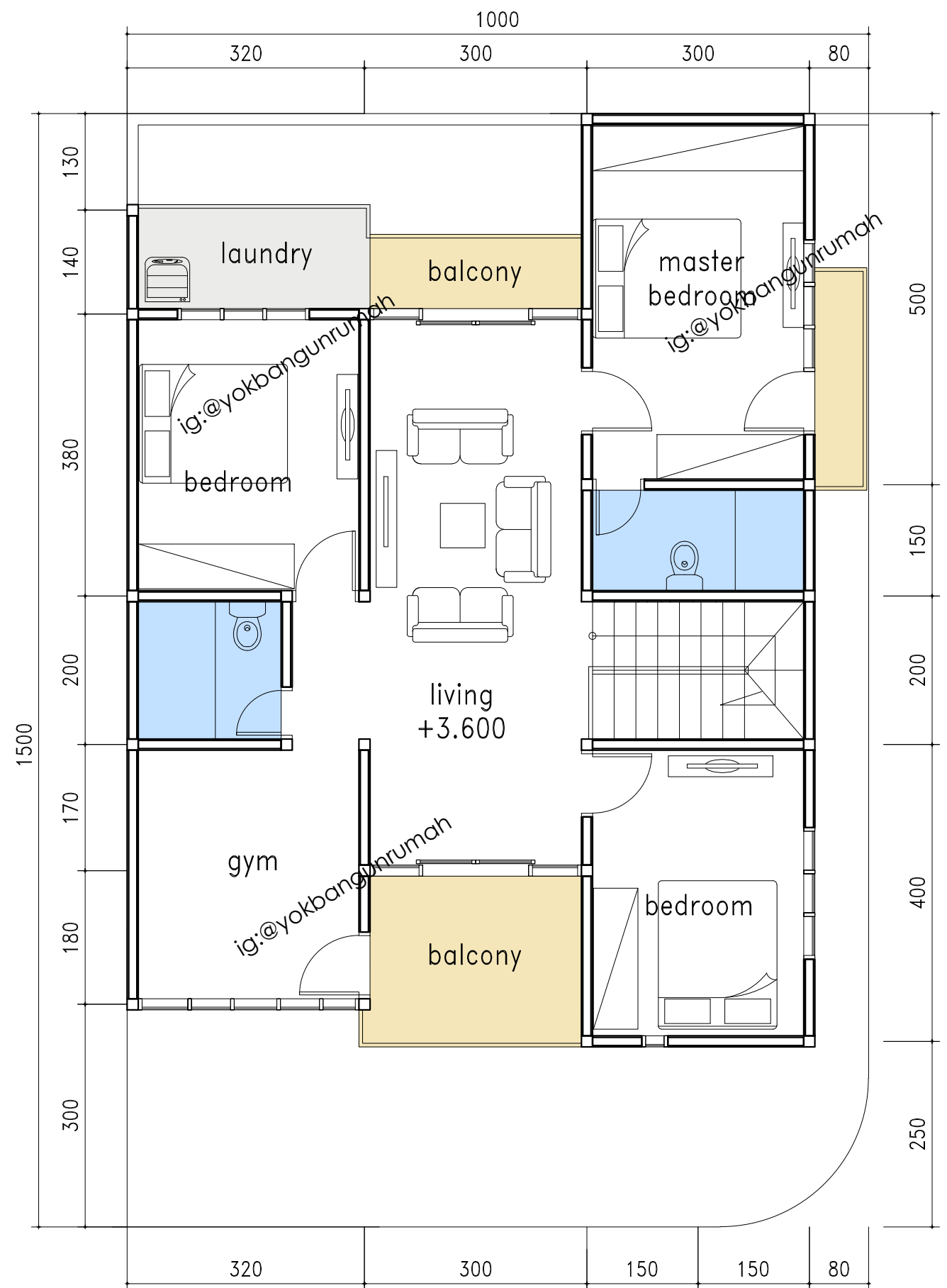
2nd FLOORPLAN
