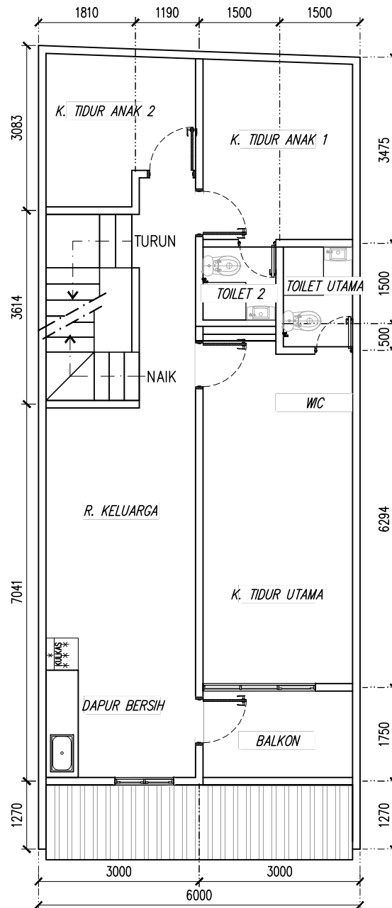
DENAH LT. 2
