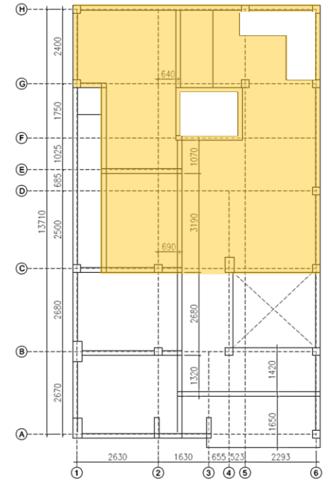
Lantai Lt II
