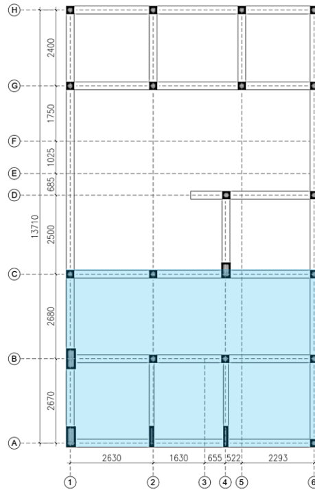
Denah Balok Lt 2
