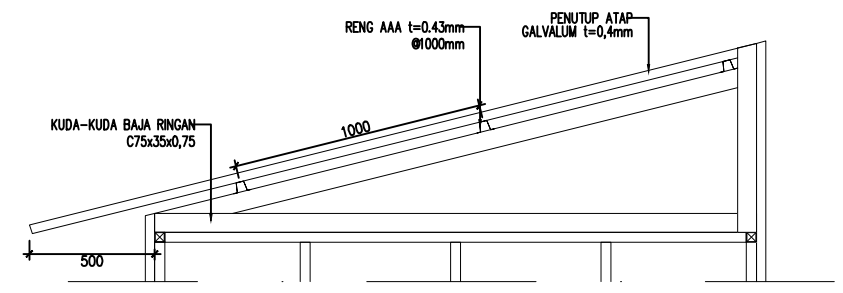
DETAIL ATAP R.LIMBAH
