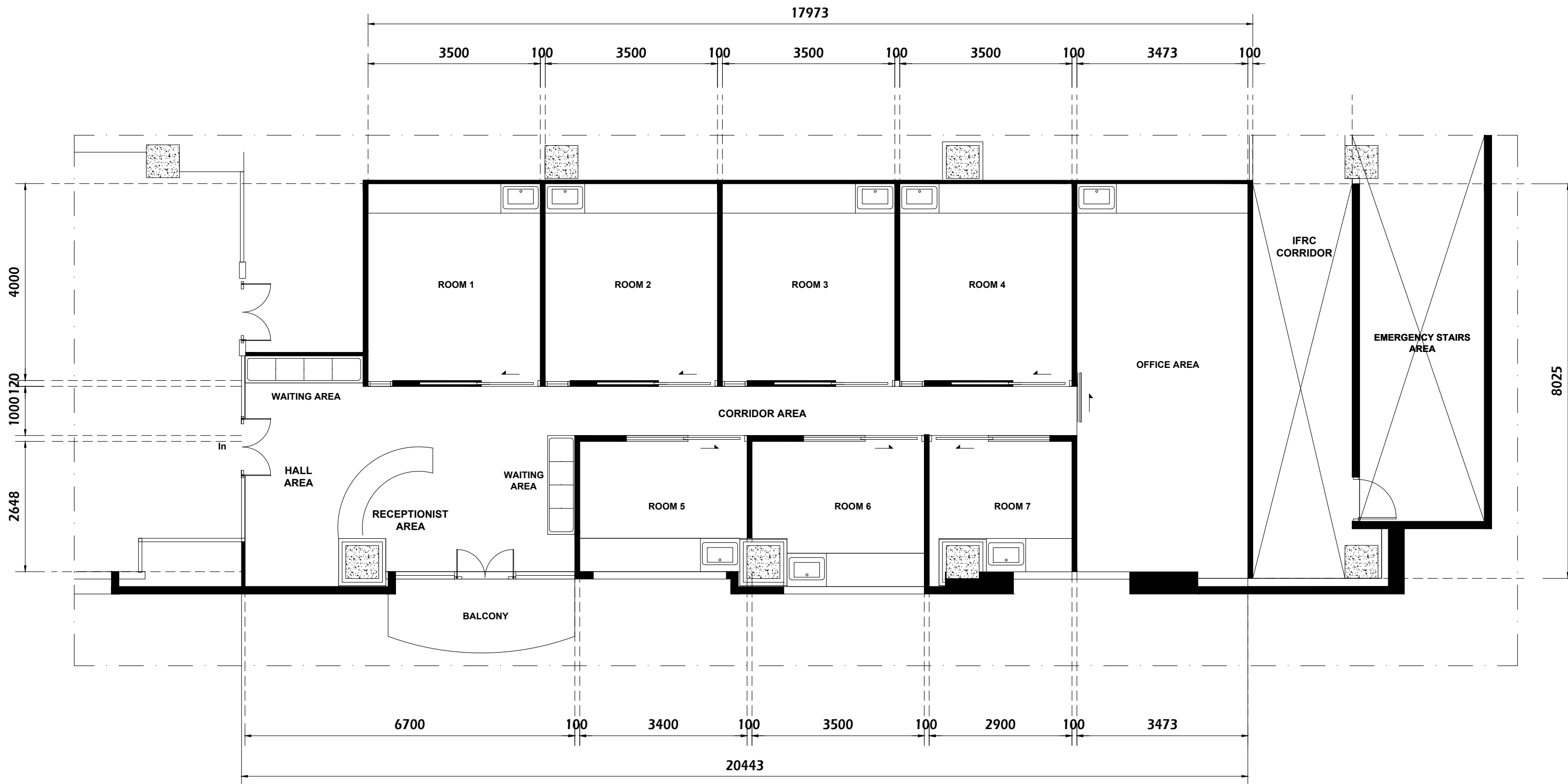
LAYOUT LANTAI 5
